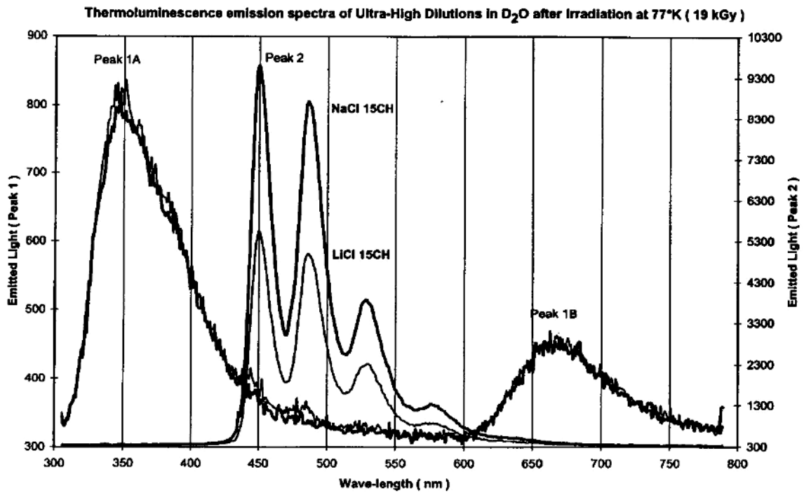
Fig. 9. Thermoluminescence emission spectra of ultra-high dilutions in D 2 O after irradiation at 77°K ( 19 kGy).
